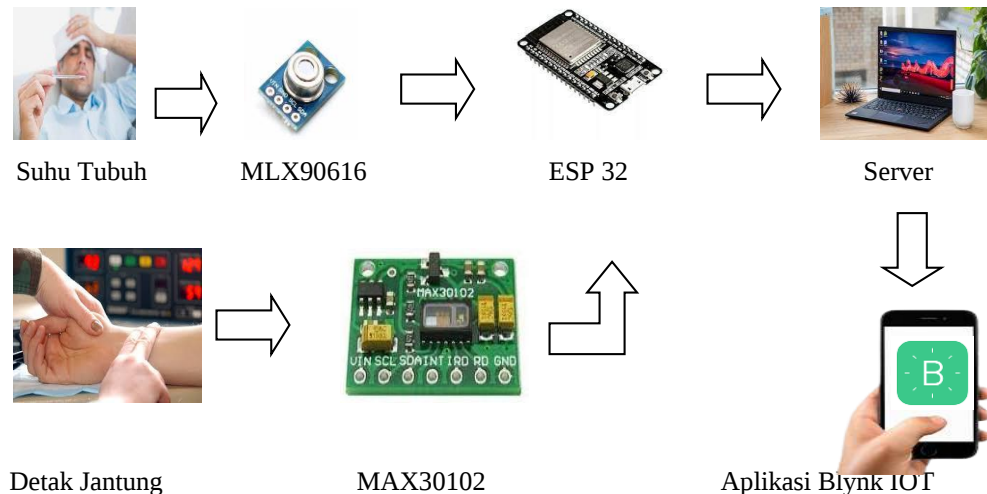
Gambar 2. Blok Diagram
