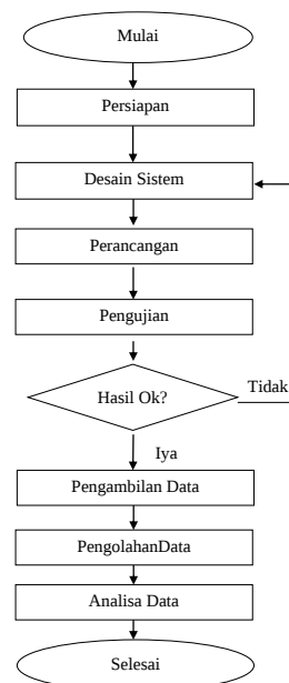
Gambar 1. Flowchart Penelitian
